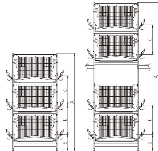
Cage for layer breeder with natural service mode (chain feeding)
