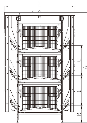
Cage for laying breeder chicken with natural service mode (hopper feeding)
